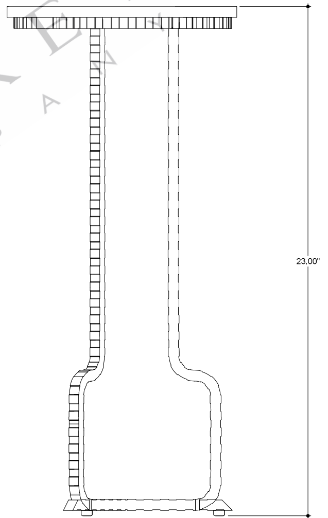
SIDE VIEW
